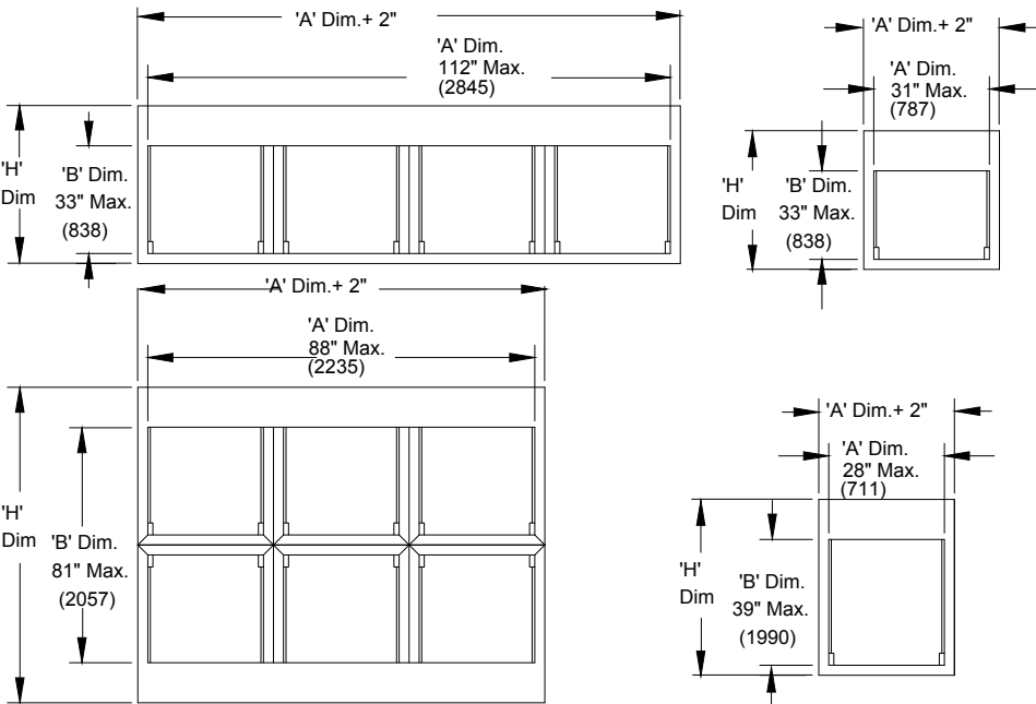
Typical Style CO and WO Construction
