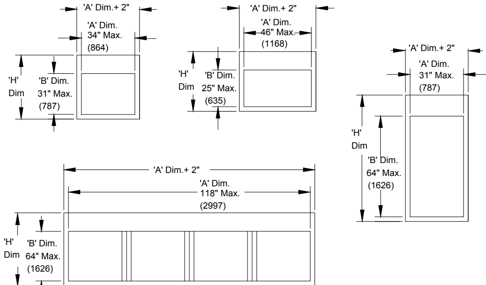
Typical Style C and WC Construction
