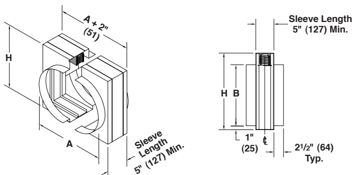
LO Style Without Sleeve
